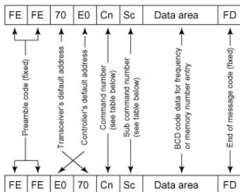
IC-7000 TO CONTROLLER
