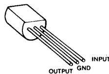
TA78L005AR IC6 (3-TERMINAL 5V REGULATOR)
