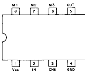
μPB555C IC3 (2-MODULUS PRESCALER)
