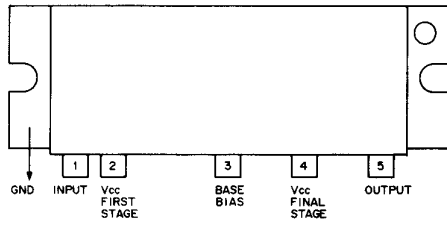
SC-1013 IC1 (POWER MODULE)
