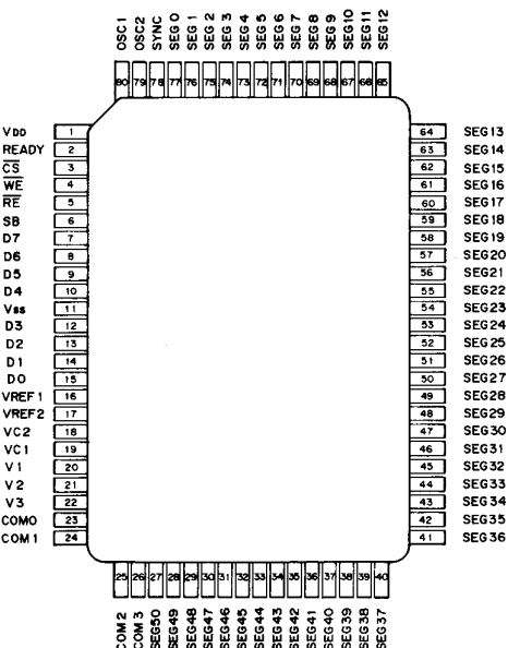
HD61602 IC3 (LCD DRIVER)
