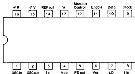
MC145158P1 IC2 (SERIAL INPUT PLL FREQUENCY SYNTHESIZER)
