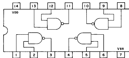
μPD4011BC IC2 (QUAD 2-INPUT POSITIVE NAND GATE)
