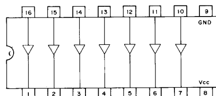
BA618 IC17 (DRIVER)
