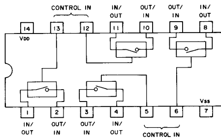
μPD4066BC IC1 (QUAD BILATERAL SWITCHING)
