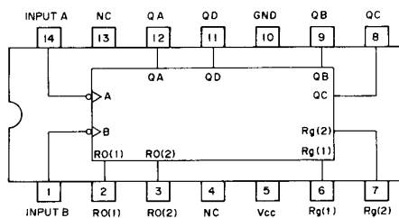
SN74LS90N IC4 (DECADE COUNTERS)
