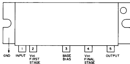
SC-1020 IC1 (POWER MODULE)
