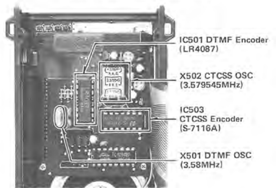
TONE UNIT (IC-04AT only)
