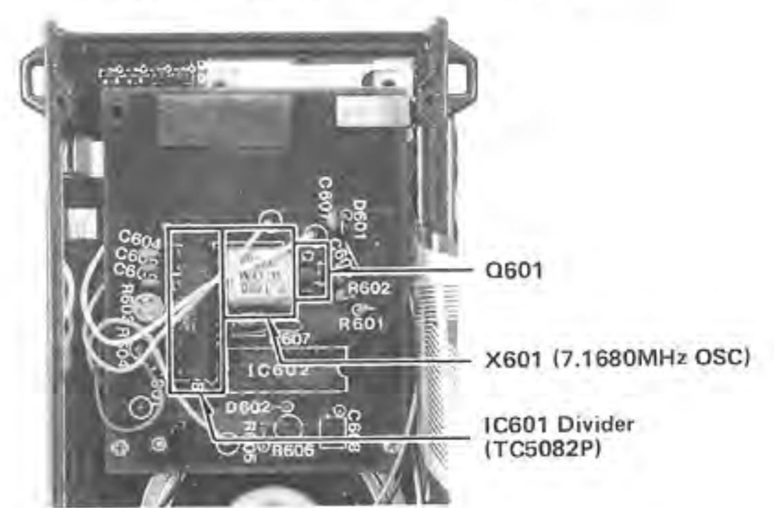
TONE CALL UNIT (IC-04E only)
