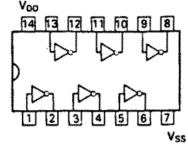
TC4069UBP (Hex Inverter) IC103
