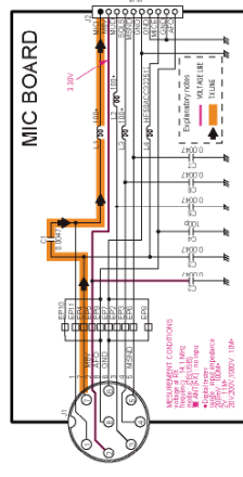
11-7 MIC BOARD
