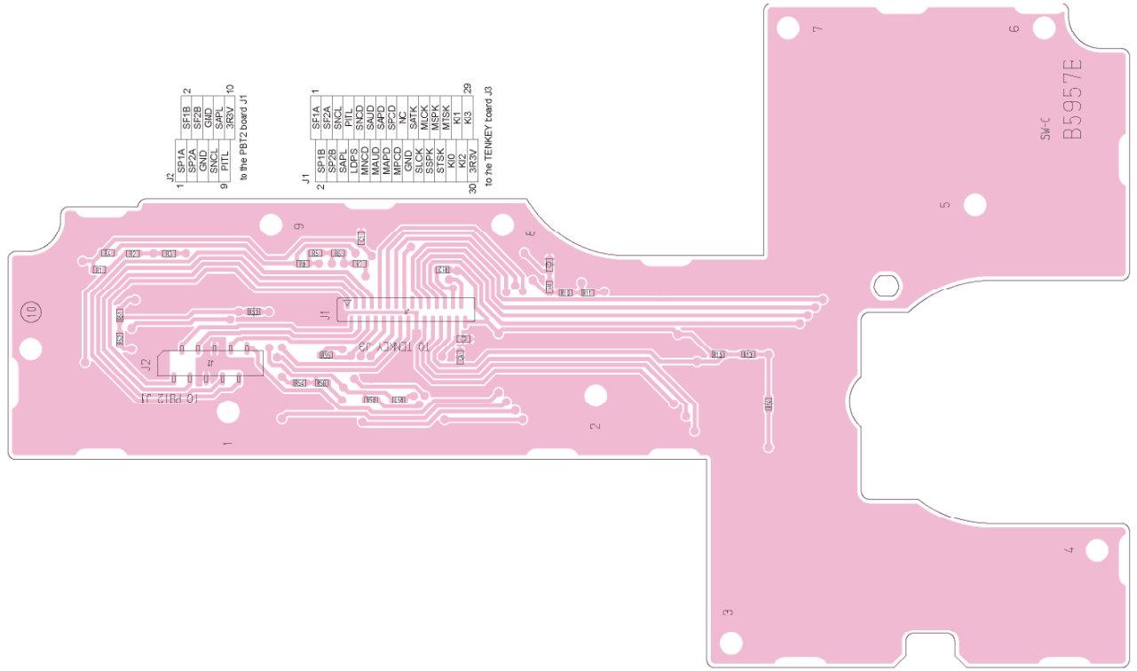
• BOTTOM VIEW (SW-C BOARD)
