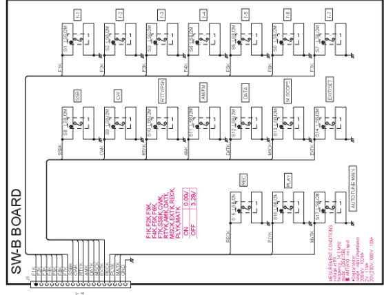
11-10 SW-B BOARD
