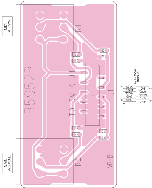
8-6 VR-B BOARD • TOP VIEW
