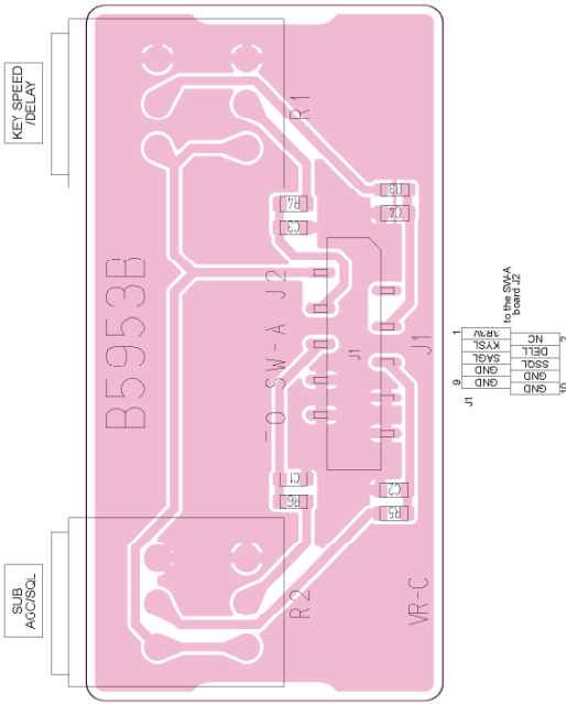
8-7 VR-C BOARD • TOP VIEW
