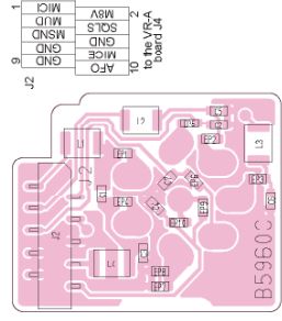
• BOTTOM VIEW (MIC BOARD)
