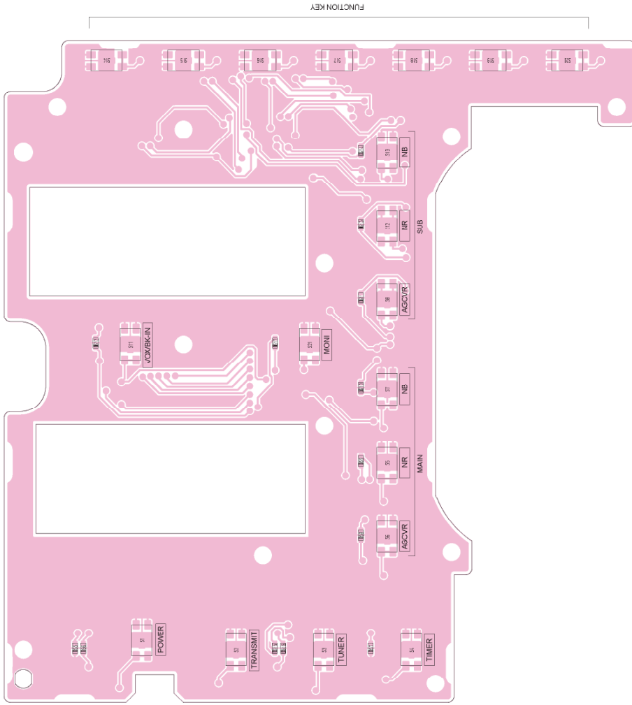
8-2 SW-A BOARD • TOP VIEW
